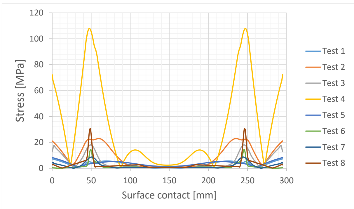
Figure 6: Von Mises yield criterion at the EP-BPP interface with hyperelastic GDL
