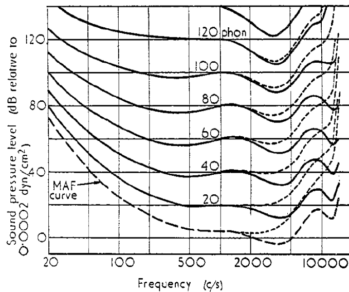
Fig. 8. Equal-loudness contours
