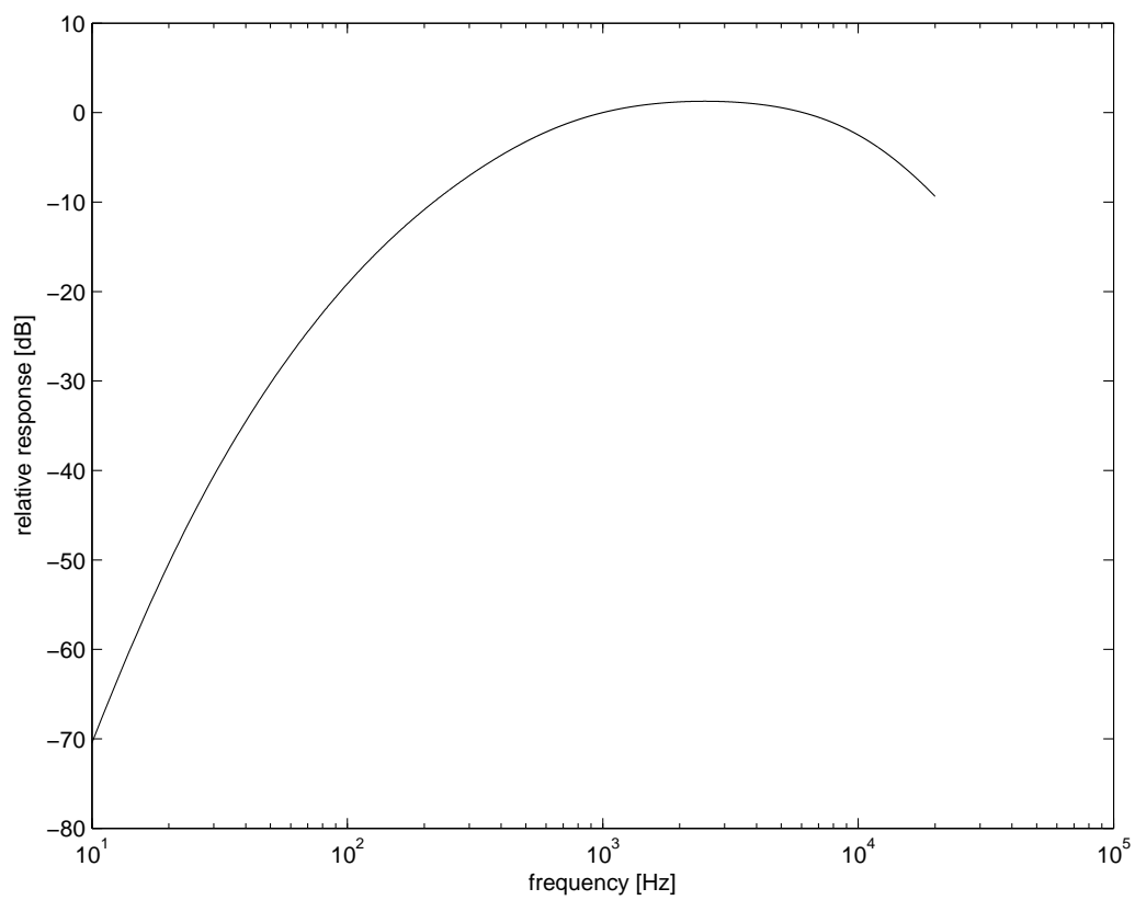
Figure 12.1: A-weighting curve.
