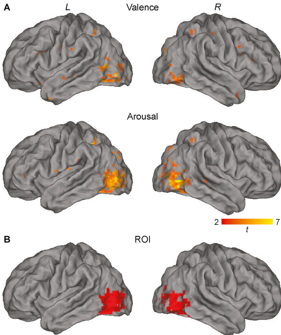
Fig. 4. (A) Statistical parametric maps thresholded at p < .001 uncorrected. (B) Bilateral regions of interest, defined by the union of voxels from the two statistical maps.
