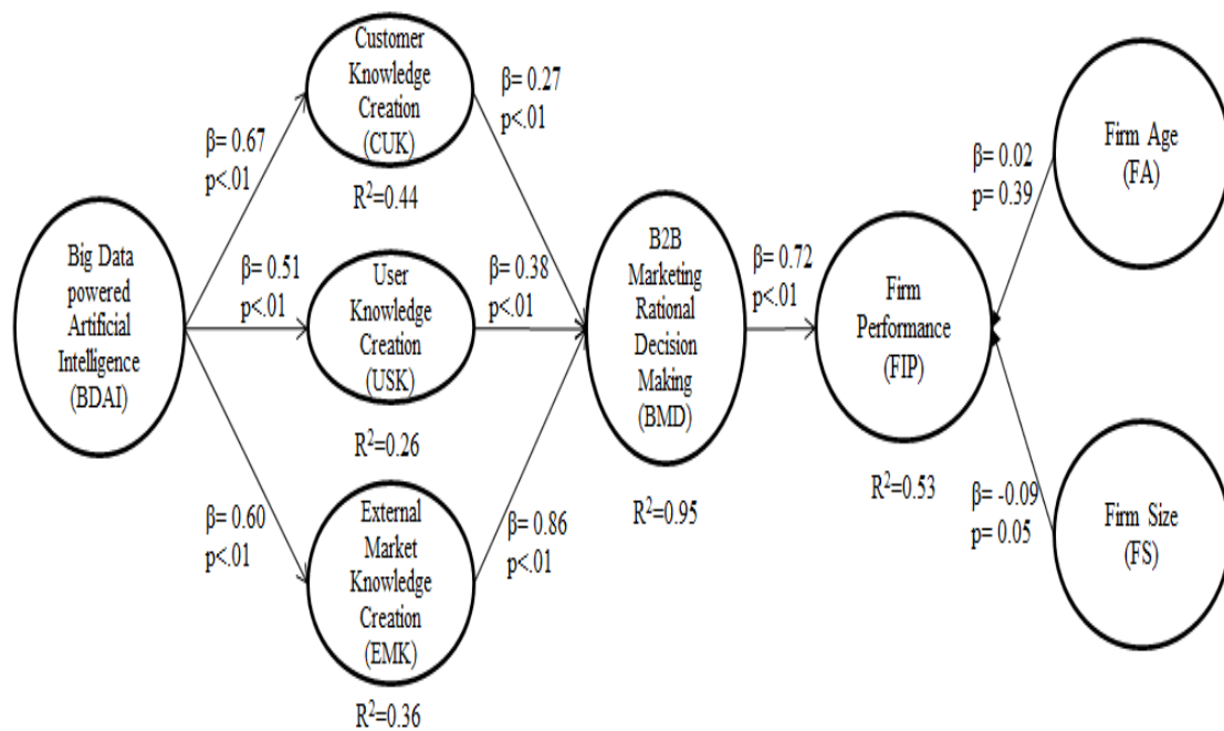
Figure 2. Model after PLS-SEM analysis
