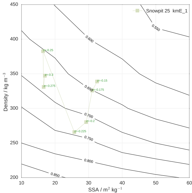
Figure 12. Ratio at 50 cm depth (black contour lines) between the radiances calculated by MCML simulations with rod and without rod for a homogeneous snowpack with varying SSA and density. Low values of the ratio indicate high rod absorptions. Green symbols represent the couples (SSA, density) at several depths measured in the 25kmE_1 snow pit.
