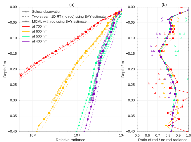
Figure 15. Same as Fig. 14 except that the simulations at 400 and 500 nm use the BAY estimate of the ice absorption coefficient.
