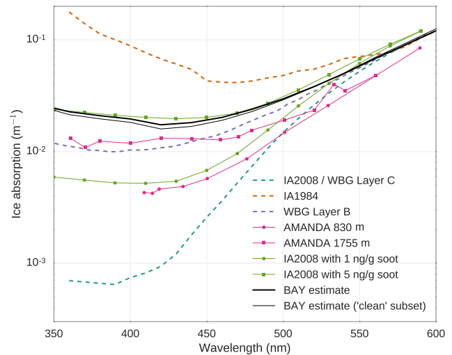
Figure 17. Estimates of ice absorption from this paper (black, BAY) from AMANDA experiment (Ackermann et al., 2006) (pink) and from Warren et al. (2006) (blue, green, maroon). Simulations (green) show absorption of snow contaminated with soot and considering IA2008 for pure ice.
