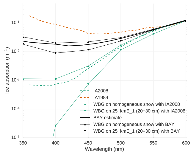
Figure 16. Ice absorption estimated with the WBG method applied to simulated irradiance profiles with MCML in the presence of the rod for the homogeneous snowpack (triangles up) and the 25kmE_1 snow pit (triangles down) by using IA2008 (green) and BAY (black) ice absorption spectra, respectively, as input.
