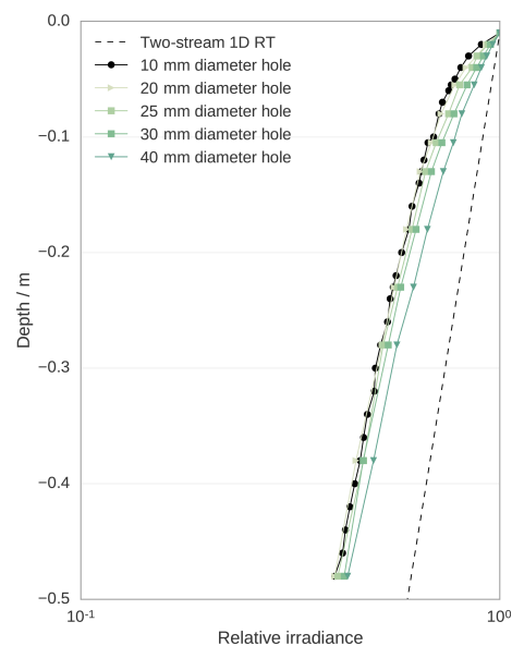
Figure 11. Influence of the air gap between the 10 mm diameter rod and snow simulated with MCML at 400 nm for a homogeneous snowpack with SSA of 30 \text{ m}^2 \text{ kg}^{-1} and density of 350 \text{ kg m}^{-3} . The 1-D model shows the reference profile in the ideal case (no rod and no gap).
