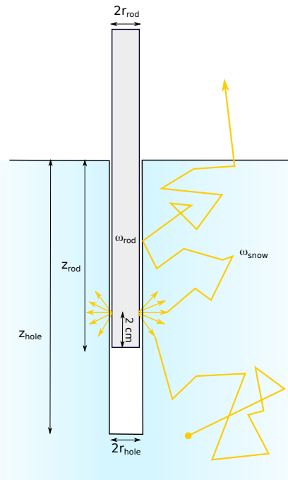
Figure 3. Principle of the 3-D radiative transfer model MCML adapted to snow. The rod (gray) is a cylinder of diameter 2r_{\text{rod}} inserted down to z_{\text{rod}} depth in the hole. The hole is also a cylinder of diameter 2r_{\text{hole}} and extends up to z_{\text{hole}} depth in the snow. Rays (orange) are launched from the sensor entrance, which is located 2 cm above the end of the rod and backpropagated. They eventually reach the surface or are discarded when their energy is lower than a small portion of its initial value ( 10^{-5} ).
