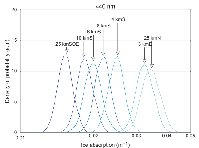
Figure 8. Posterior of ice absorption at 440 nm independently estimated on different sites by the BAY method.
