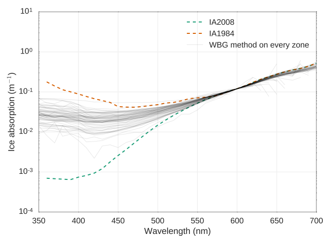
Figure 5. Seventy ice absorption spectra estimated by the WBG method (Warren et al., 2006) on each homogeneous zone from the selection on the 56 radiance profiles measured around Concordia.
