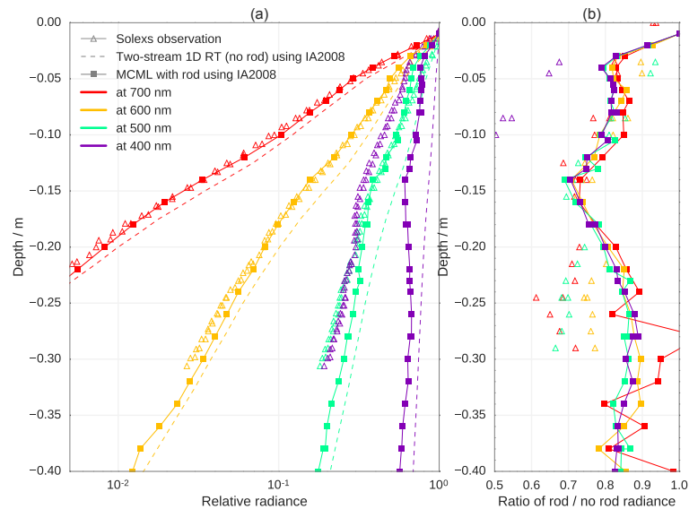
Figure 14. Log-radiance profiles at 400, 500, 600, and 700 nm measured by SOLEXS at 25kmE_1 (25 km east of Concordia). Simulations with the 1-D model TARTES (without rod) and the 3-D model MCML using density and SSA profiles measured at the same point (Libois et al., 2014b). (b) Same as (a) but normalized by the ideal case computed with TARTES.
