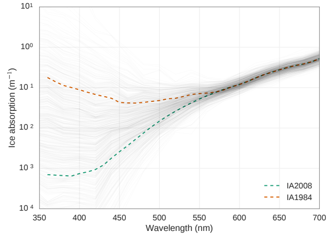
Figure 2. Samples (gray) of the prior distribution of the ice absorption to be used by the BAY method. Ice absorption coefficients IA1984 and IA2008 are presented for reference.
