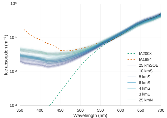
Figure 7. Ice absorption estimated by the BAY method at different locations around around Concordia.
