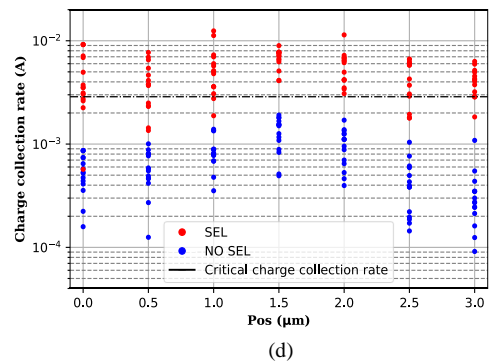
Fig. 16 Charge collection rate using the second criterion at 350 K (a), 375 K (b), 400 K (c) and 425 K (d).
