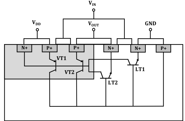
Fig. 2 Full CMOS inverter structure and the Latchup paths.
