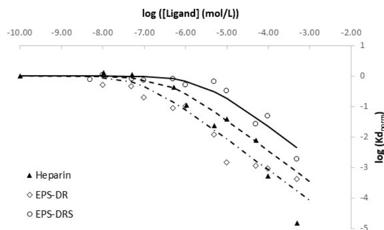
Figure 6. Ligand concentration isotherms of EPS-DR, EPS-DRS and Heparin: pH = 6.1 \pm 0.1 ; 10 mg of chelex 100 resin in 5 mL of solutions; [\text{Sc}^{3+}] = 10^{-4} \text{ mol L}^{-1} , [EPS-DR], [EPS-DRS] and [Hep] ranged from 10^{-10} to 5 \cdot 10^{-4} \text{ mol L}^{-1} .
