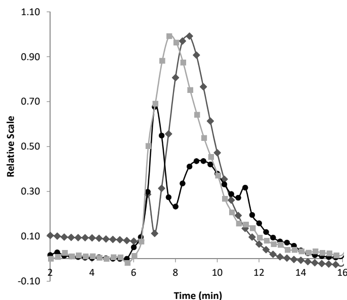
Figure 3. Fractogram of EPS-DRS (squares: UV-VIS @ \lambda = 254 nm; circles: dRI; diamonds: MALS @ 90^\circ ). [EPS-DRS] = 2 \text{ mg mL}^{-1} ; injection volume = 20 \text{ }\mu\text{L} ; eluent = MilliQ water with 0.1% in volume of Tween 20; membrane = PES 5 kDa; canal length = 291 mm; spacer = 350 \text{ }\mu\text{m} ; cross flow = from 2 to 0 \text{ mL min}^{-1} in 17 min; injection flow = 0.20 \text{ mL min}^{-1} ; focalization flow = 2 \text{ mL min}^{-1} ; detector flow = 1 \text{ mL min}^{-1} .
