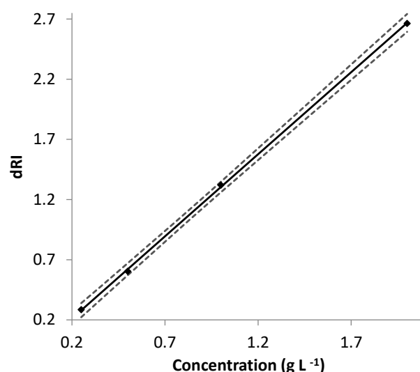
Figure 2. Determination of \partial n/\partial c of EPS-DR in ultra-pure water at 25 °C; \lambda_0 = 660 nm. Concentrations of EPS = 0.25 – 2 mg mL -1 . Measured differential refractive index dRI values ( \times 10^4 ) with EPS-DR concentration. The solid line represents the linear fit; the uncertainties' hyperboles are plotted in dashed lines.
