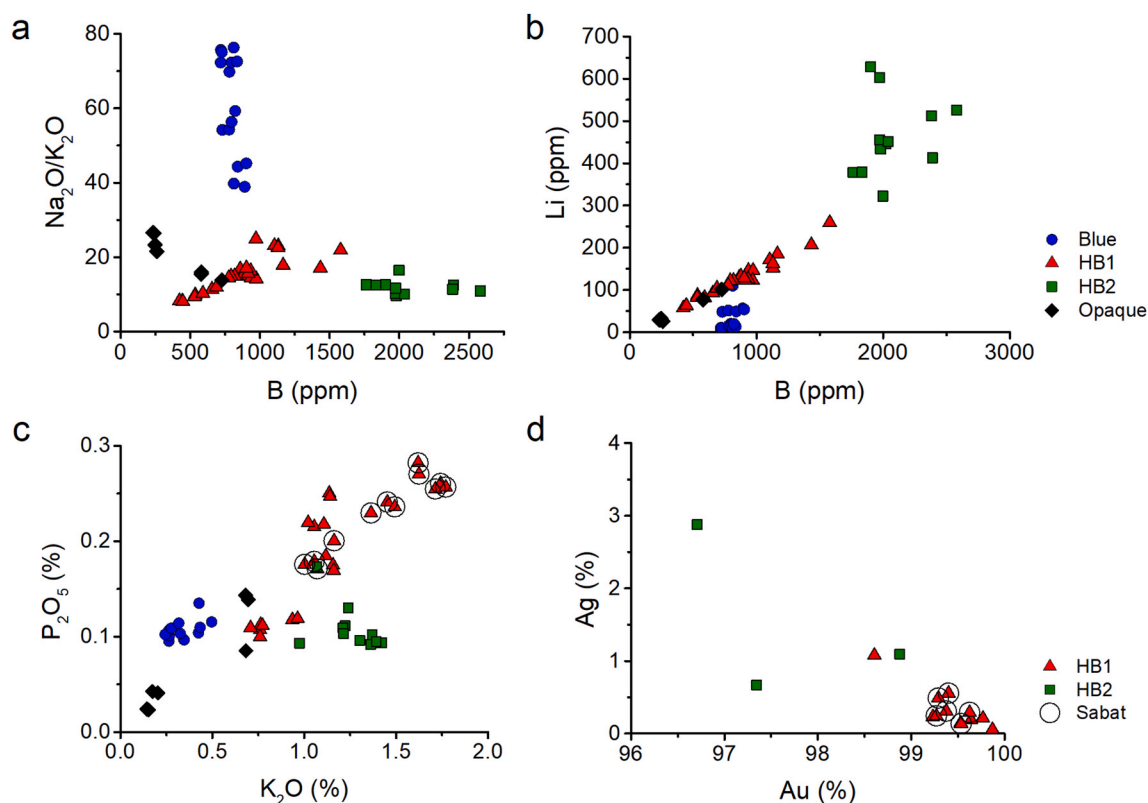
Fig. 2. Compositional characteristics of the different high boron groups (LA-ICP-MS). (A) \text{Na}_2\text{O}/\text{K}_2\text{O} ratios versus boron show a clear difference between the fluxes; (B) lithium and boron are positively correlated in the high B1, high B2 and opaque glasses; (C) \text{K}_2\text{O} and \text{P}_2\text{O}_5 are elevated in the high B1 group possibly due to a batch contamination or an addition of plant ash. The circled data points represent gold leaf tesserae of the HB1 group from the Sabat door mosaic. (D) Gold leaf composition of the high boron glasses ( \mu -PIXE). Gold versus silver contents show different compositions that match with the two sub-groups of high boron glasses. (For interpretation of the references to colour in this figure legend, the reader is referred to the Web version of this article.)
