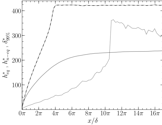
Figure 21: Evolution of h_{eq}^* , h_{n-eq}^* and \delta_{99\%}^* along the channel flow: \cdots\cdots h_{eq}^* ; -\cdot-\cdot- h_{n-eq}^* ; — \delta_{99\%}^* .
