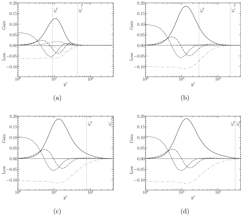
Figure 24: Budgets of enthalpy variance at x/\delta = 0.73 (a), 2\pi (b), 5.7\pi (c) and 16.5\pi : — streamwise ( V_x : gray) and wall-normal ( V_y : black) production; - · - · - · - molecular dissipation III ; - - - - streamwise ( II_x : gray) and wall-normal ( II_y : black) molecular diffusion; - · - · - streamwise ( VI_x : gray) and wall-normal ( VI_y : black) turbulent diffusion; · · · · · streamwise ( I_x : gray) and wall-normal ( I_y : black) mean convective terms.
