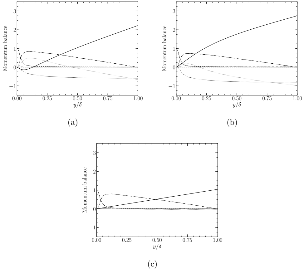
Figure 17: Momentum flux balance at x/\delta = -0.06 (a), 0.18 (b), and 5\pi (c): — pressure gradient; - - - streamwise (gray) and wall-normal (black) viscous terms; \cdots streamwise (gray) and wall-normal (black) mean convective terms; - \cdot - \cdot - streamwise (gray) and wall-normal (black) turbulent terms.
