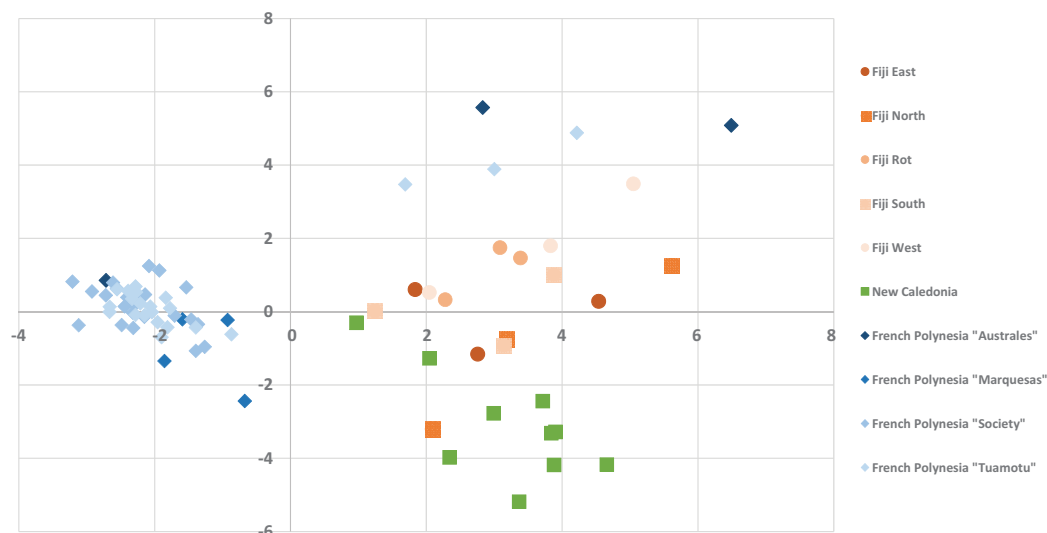
Figure 5 The PCA Scatter plot revealing the chemical diversity of C. inophyllum within the three study areas. The first two components correspond to 15.81% and 7.59% of the total variance respectively. Orange circles for Fiji, green squares for New Caledonia and blue diamonds for French Polynesia.
