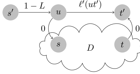
Figure 1: Digraph D' defined from D (Theorem 2) with \ell'(ut') = 1 for the Min measure and \ell'(ut') = 0 for the Max and Jaccard measures.
