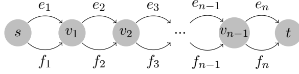
Figure 2: Digraph D_S = (V, A) defined from \mathcal{S} = \{x_1, \dots, x_n\} . For all 1 \leq i \leq n , \ell(e_i) = x_i . For all 1 \leq i \leq n , we have \ell(f_i) = x_i in the proof of Theorem 3 and \ell(f_i) = M \cdot x_i with M > 1 in the proof of Theorem 4.
