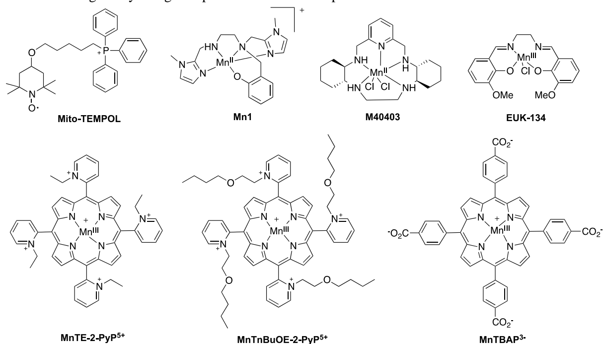
Figure 1. Structure of the selected antioxidants studied in this article.
