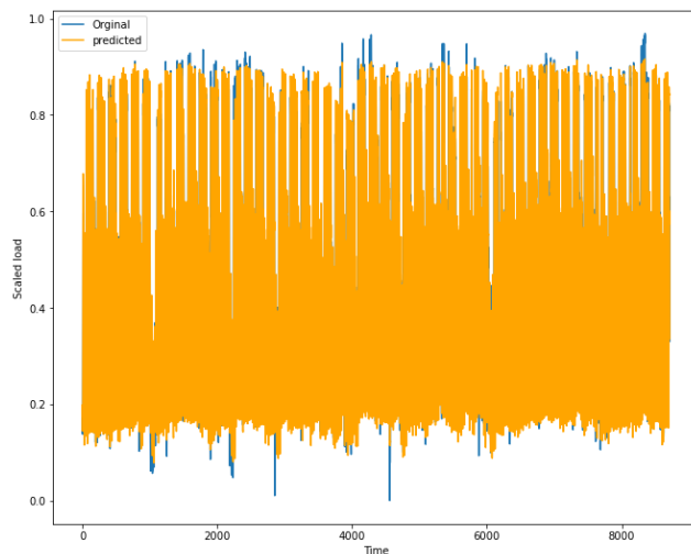
FIGURE 43. 10 days ahead results using the PLCNet, Malaysian data.
