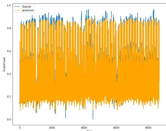
FIGURE 42. 2 days ahead results using the PLCNet, Malaysian data.
