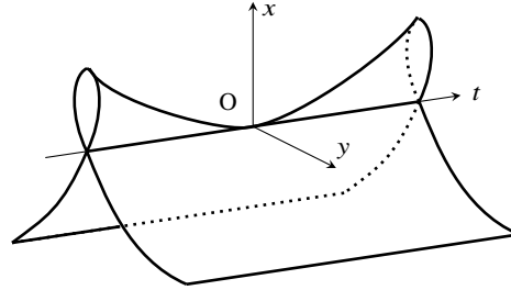
Fig. 3: y^2 = t^2 x^2 - x^3 = 0
