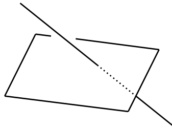
Fig. 2: z(x^2 + (y + z)^2) = 0
