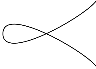
Fig. 1: y^2 = x^2 + x^3 = 0
