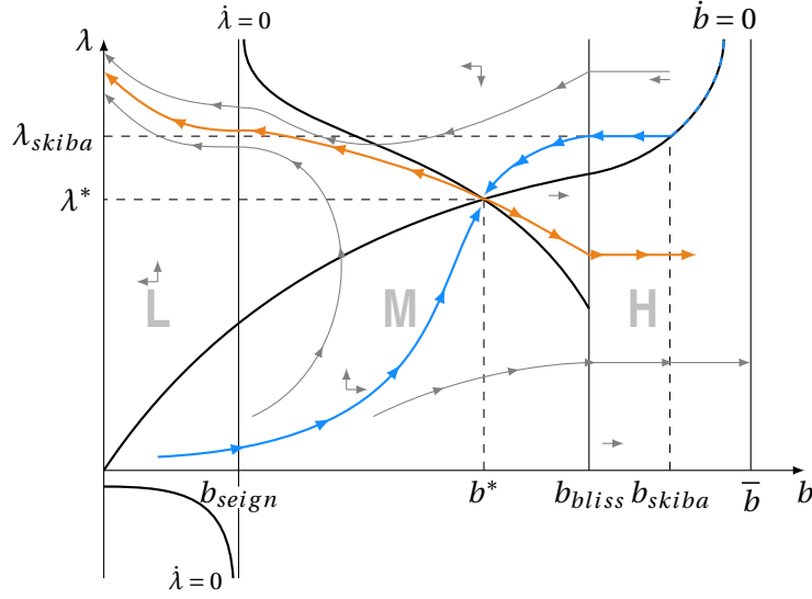
Figure 8: Benchmark, with \psi_{bliss} > \gamma_{bliss} .
