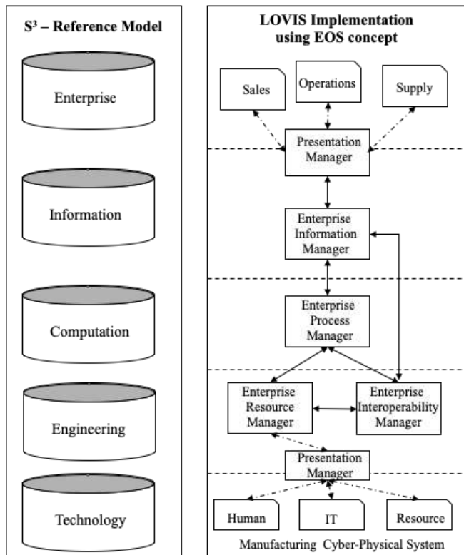
Figure 7. Implementation of an EOS System using the S^3 E-RM (Chavarría-Barrientos et al., 2018)
