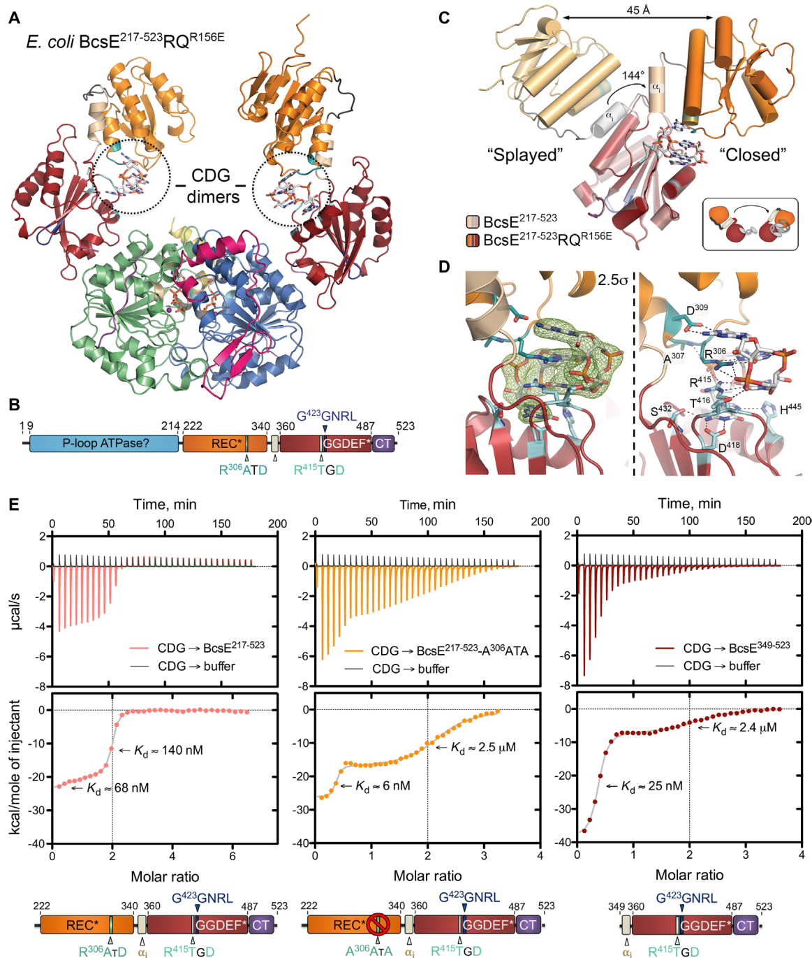
Fig. 5. Multisite c-di-GMP recognition and structure of the BcsRQ 156E -BcsE REC* -GGDEF* complex. (A) Crystal structure of untagged BcsRQ 156E -E 217-523 assembly in complex with ATP/ACP ( \beta,\gamma -methyleneadenosine triphosphate or AppCp) and c-di-GMP. (B) Full-length BcsE domain architecture and functionally validated c-di-GMP-binding motifs (RxxD I-sites I and II) as identified in this study. (C) Captured conformational changes in the BcsE REC*-GGDEF* tandem between the BcsE 217-523 ["Splayed" (10)] and BcsRQ 156E -E 217-523 ("Closed") crystal structures. (D) Close-up views of c-di-GMP complexation in the three-component complex. Left: An |F_o| - |F_c| partial electron density map calculated from a model before inclusion of the dinucleotide and contoured at 2.5 \sigma . Right: A cartoon-and-stick representation of c-di-GMP coordination. Canonical I-site I residues are colored in cyan; secondary I-site II residues are colored in teal. (E) Functional validation of the secondary I-site on the BcsE REC* module (R 306 ATD) by isothermal titration calorimetry. K_d values were calculated using a two-site binding model.
