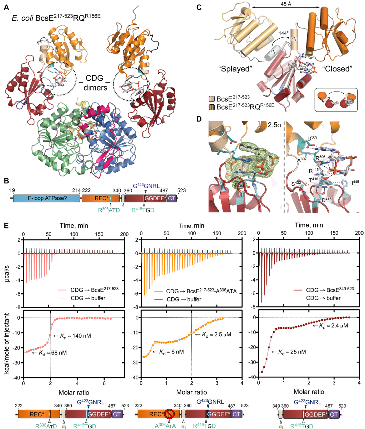
Fig. 5. Multisite c-di-GMP recognition and structure of the BcsRQ 156E -BcsE REC*GGDEF* complex. (A) Crystal structure of untagged BcsRQ 156E -E 217-523 assembly in complex with ATP/ACP ( \beta,\gamma -methyleneadenosine triphosphate or AppCp) and c-di-GMP. (B) Full-length BcsE domain architecture and functionally validated c-di-GMP-binding motifs (RxxD I-sites I and II) as identified in this study. (C) Captured conformational changes in the BcsE REC*GGDEF* tandem between the BcsE 217-523 ["Splayed" (10)] and BcsRQ 156E -E 217-523 ("Closed") crystal structures. (D) Close-up views of c-di-GMP complexation in the three-component complex. Left: An |F_o| - |F_c| partial electron density map calculated from a model before inclusion of the dinucleotide and contoured at 2.5 \sigma . Right: A cartoon-and-stick representation of c-di-GMP coordination. Canonical I-site I residues are colored in cyan; secondary I-site II residues are colored in teal. (E) Functional validation of the secondary I-site on the BcsE REC* module (R 306 ATD) by isothermal titration calorimetry. K_d values were calculated using a two-site binding model.
