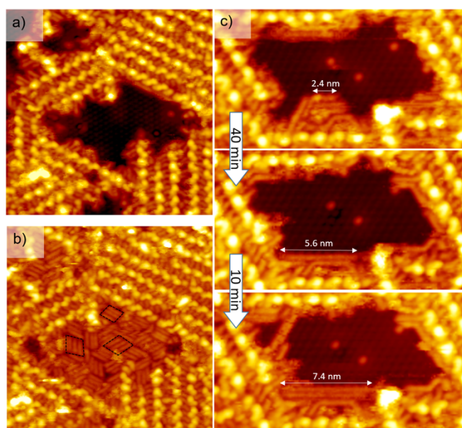
Figure 3. a) STM image ( 25 \times 25 \text{ nm}^2 , V_s = -1.3 V, I_t = 7 pA, T = 110 K) representing an nano-pore inside the supramolecular network. b) The same nano-pore fully filled with rod-like structure released by STM tip during scanning. c) Three STM images ( 10 \times 20 \text{ nm}^2 , V_s = -1.3 V, I_t = 7 pA, T = 110 K) showing the growth of rod-like structure in a nanopore.
