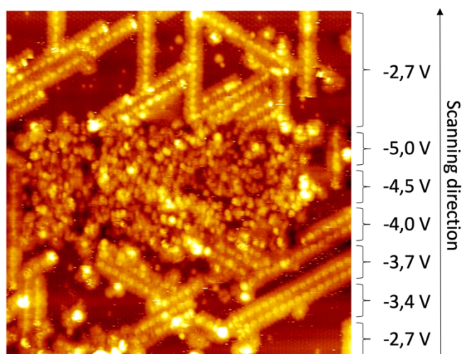
Figure 2. STM image captured while changing bias voltage during the scan shows significant modification of network at -4.5 V ( 60 \times 60 \text{ nm}^2 , V_s = variable values shown on image, I_t = 7 pA, T = 110 K).
