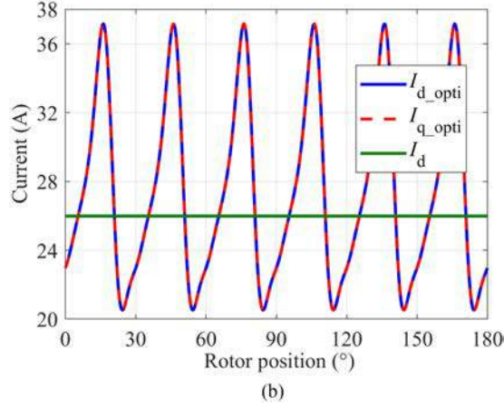
Fig. 2. Original currents and optimal currents ( \beta = 45^\circ , I_m = 30 A) of FEM. (a) Stator currents. (b) Currents of dq -axis.
