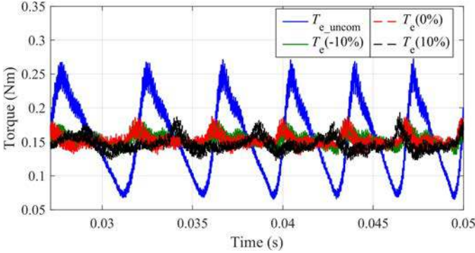
Fig. 24. Uncompensated torque and compensated torques by K_t with inertia error.
