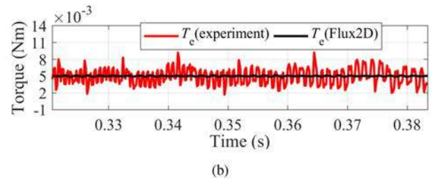
Fig. 18. Electromagnetic torque calculated in experiment. (a) Without compensation. (b) With compensation.
