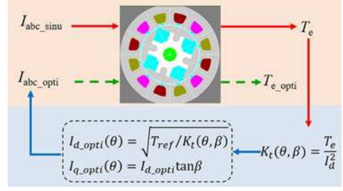
Fig. 1. Torque ripple reduction based on torque function.
