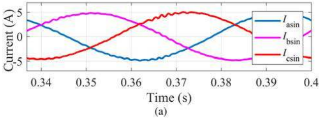
Fig. 15. Stator current in experiment. (a) Without compensation. (b) With compensation.
