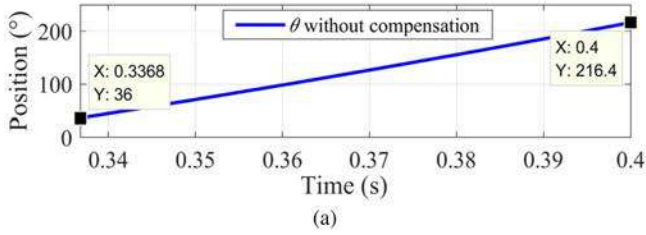
Fig. 14. Measured rotor position in experiment. (a) Without compensation. (b) With compensation.
