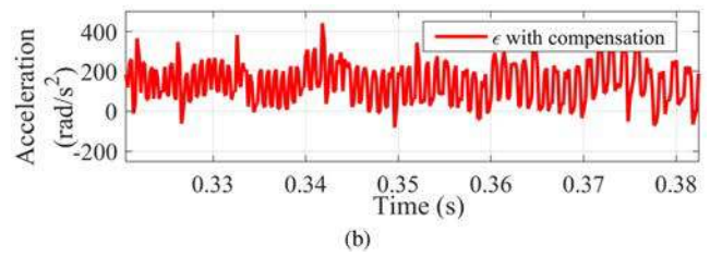
Fig. 17. Acceleration obtained by speed in experiment. (a) Without compensation. (b) With compensation.
