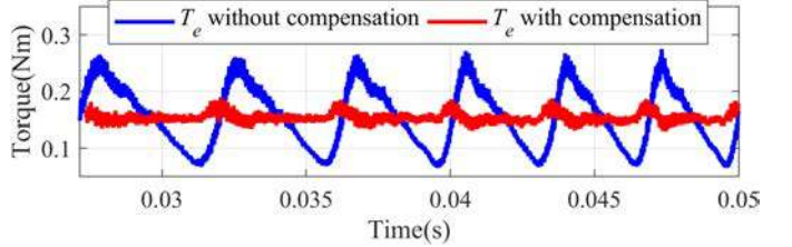
Fig. 9. Torque without compensation and with compensation.
