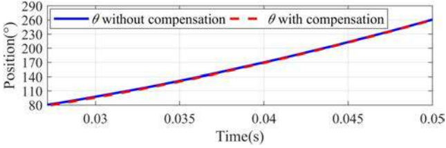
Fig. 6. Rotor position without compensation and with compensation.
