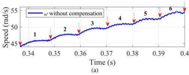
Fig. 16. Rotor speed calculated by position in experiment. (a) Without compensation. (b) With compensation.
