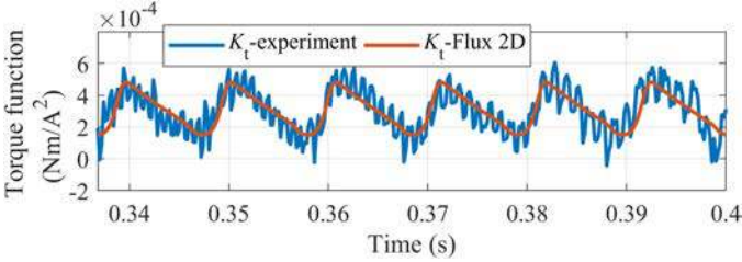
Fig. 20. Torque functions obtained by experiment and FEM.
