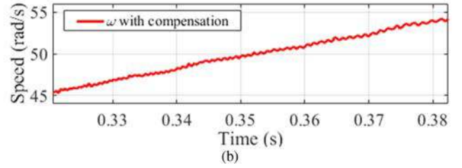
Fig. 16. Rotor speed calculated by position in experiment. (a) Without compensation. (b) With compensation.
