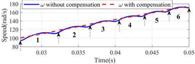
Fig. 7. Rotor speed without compensation and with compensation.
