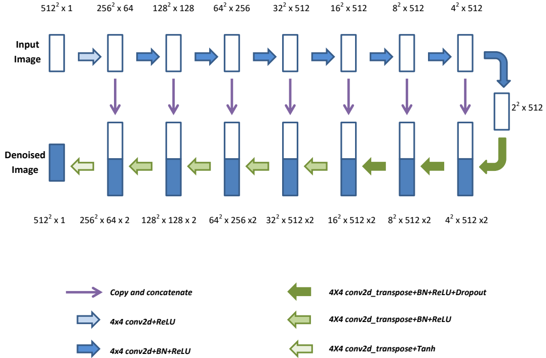
Figure 2: Schematic diagram of the Fully Convolutional Neural Network based Denoising [19].
