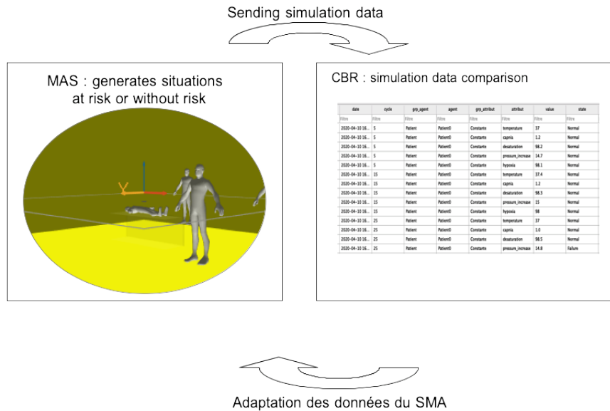
Fig. 1: MAS/CBR exchanges
