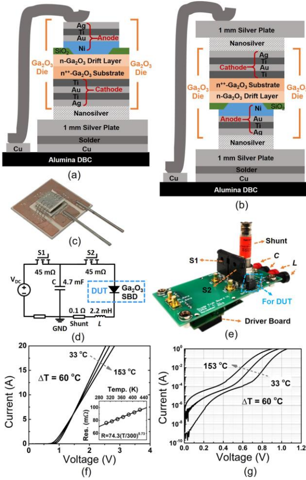
Fig. 1. Schematic of the Ga 2 O 3 SBDs with (a) bottom-side-cooling package and (b) double-side-cooling package. (c) Photo of a double-side-cooled SBD. (d) Circuit diagram and (e) photo of the surge current test board. Forward I-V characteristics of the packaged Ga 2 O 3 SBDs at 33–153 °C in the (f) linear region and (g) subthreshold region. [inset of (f)] temperature-dependence of the differential R_{on} and the power law fitting.
