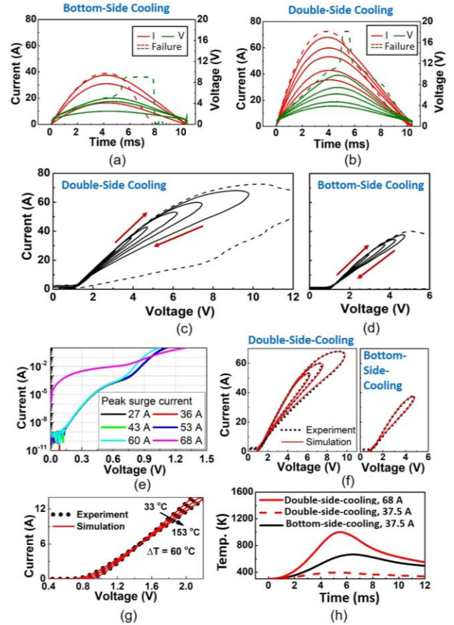
Fig. 2. Current/voltage waveforms of the (a) bottom-side-cooled and (b) double-side-cooled Ga 2 O 3 SBDs in the surge current tests. I-V loops of the (c) double-side-cooled and (d) bottom-side-cooled devices. (e) Transfer characteristics in the subthreshold region after each surge current test. Simulation model calibration for the (f) surge I-V loops and (g) static I-V characteristics. (h) Simulated junction temperature in the surge current tests for bottom-side-cooled and double-side-cooled Ga 2 O 3 SBDs.
