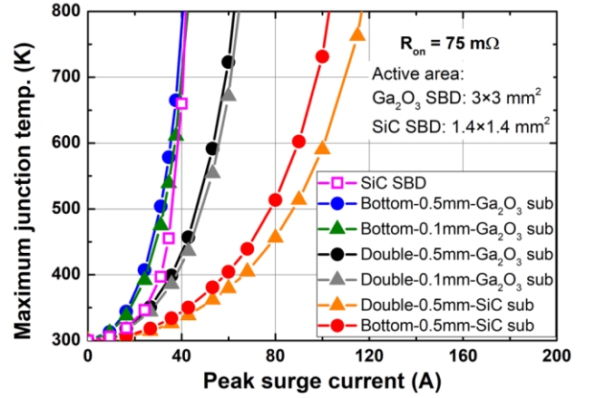
Fig. 4. Simulated max junction temperature as a function of peak surge current in 10-ms surge tests for the double-side-cooled and bottom-side-cooled Ga 2 O 3 SBDs on the 0.5-mm-thick Ga 2 O 3 substrate, 0.1-mm-thick Ga 2 O 3 substrate, and 0.5-mm-thick SiC substrate. A thermal boundary resistance of 0.01 K/(W·cm 2 ) was set at the Ga 2 O 3 /SiC bonding interface. Identical electrical conductivity was set for Ga 2 O 3 and SiC substrates. The simulated SiC SBD has a 0.5-mm-thick substrate and a bottom-side-cooled package. Caughey-Thomas model was used for the SiC electron mobility.
