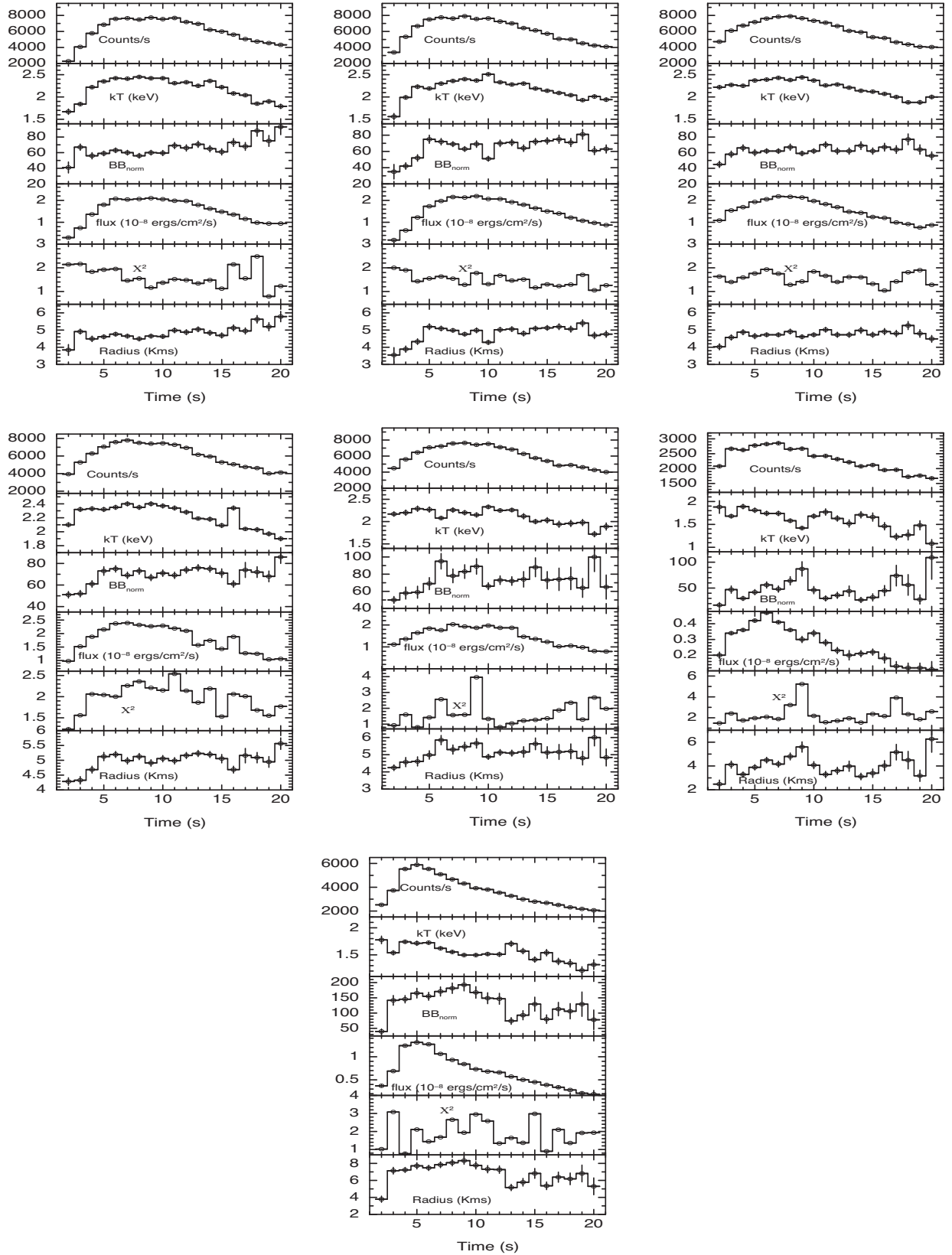
Figure 8. First panel: in the left we show the best-fitting parameters obtained after performing time-resolved spectroscopy of burst 1. We have not applied correction factors to obtain a real value of the NS radius. Middle: best-fitting parameters obtained after performing time-resolved spectroscopy of burst 2 and the right plot shows the best-fitting parameters obtained from the time-resolved spectroscopy of burst 3. Second panel: In the left we show the best-fitting parameters obtained after performing time-resolved spectroscopy of burst 4, the plot in the middle is for burst 5 while the right plot is for burst 6. Third panel: best-fitting parameters obtained after performing time-resolved spectroscopy of burst 7.
