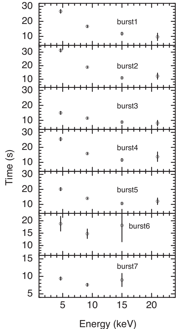
Figure 6. This plot shows an exponential decay time-scales observed in different energy bands during seven bursts observed in the LAXPC data of 4U 1636–536.
