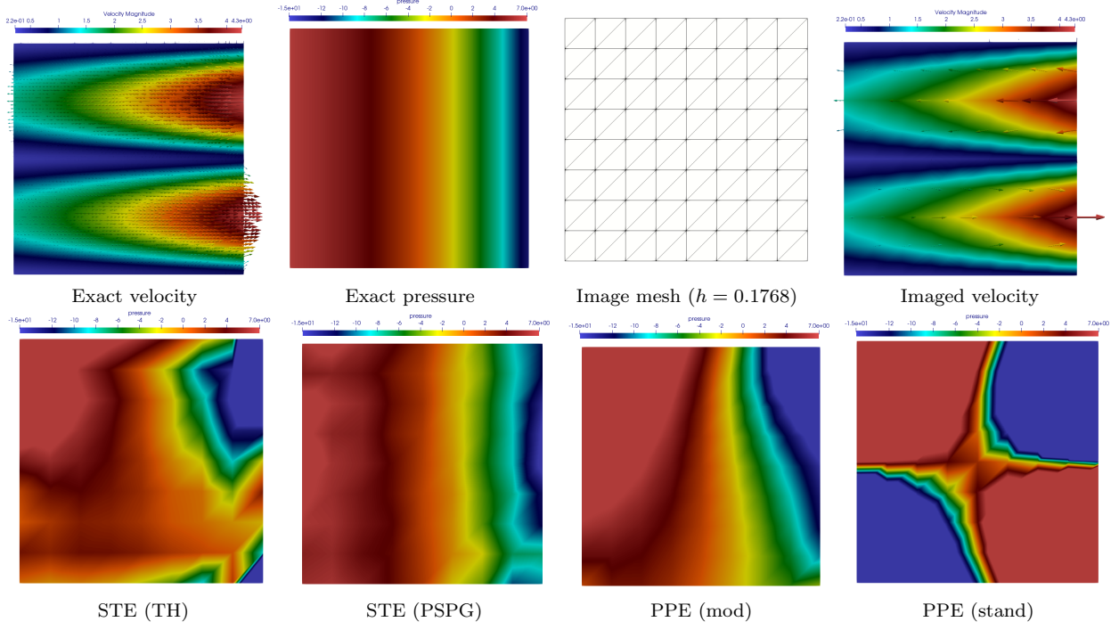
Figure 7: \mathbb{P}_1 -interpolated reference velocity and pressure fields (top) and reconstructed pressure fields with order k = 1 (bottom) for \nu = 2\pi in Example 2.
