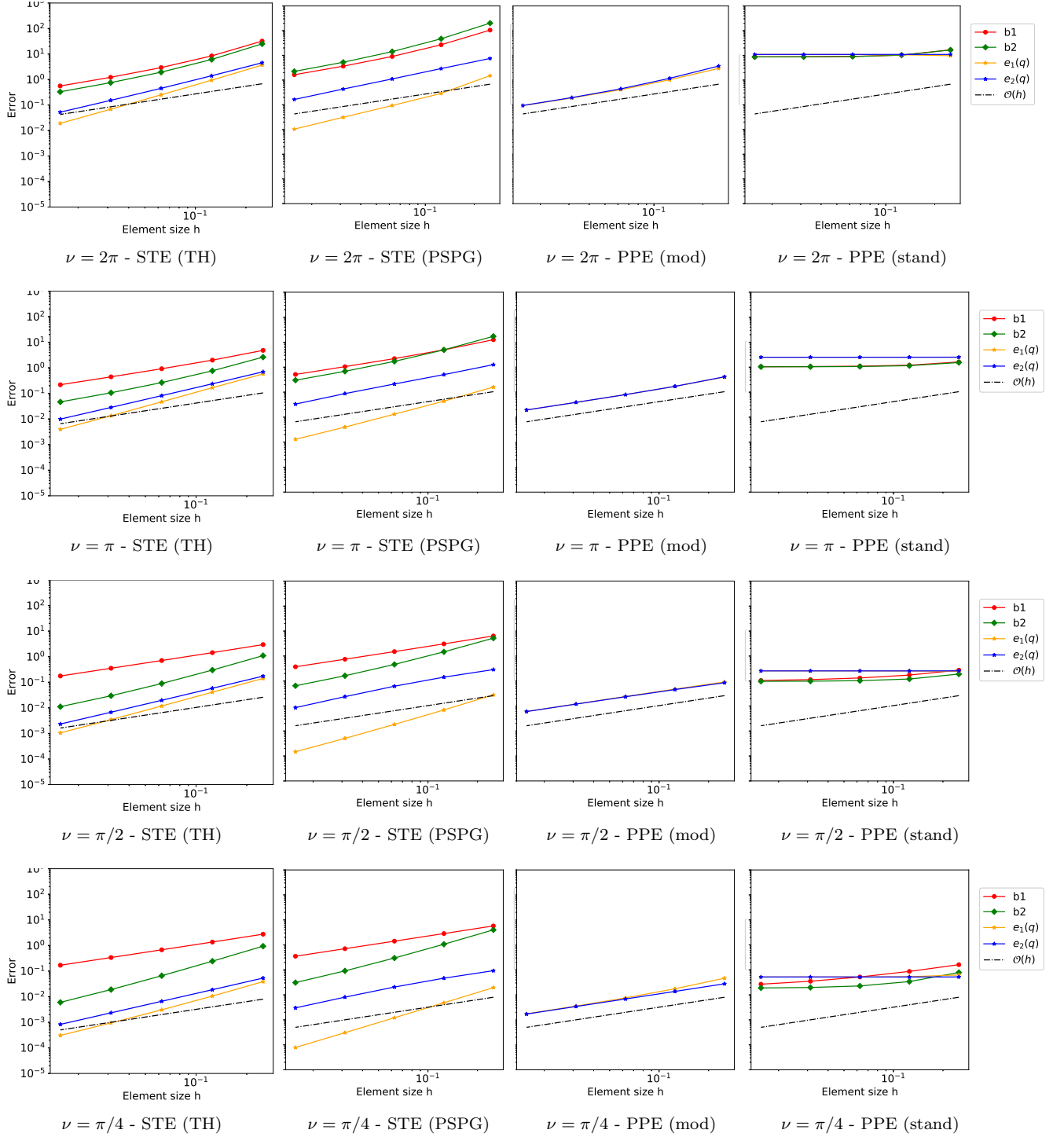
Figure 6: Pressure error curves and bounds for viscosities values \pi/4 , \pi/2 , \pi and 2\pi of Example 2. The figures for the modified PPE do not present the error bound as explained in the beginning of Section 4.
