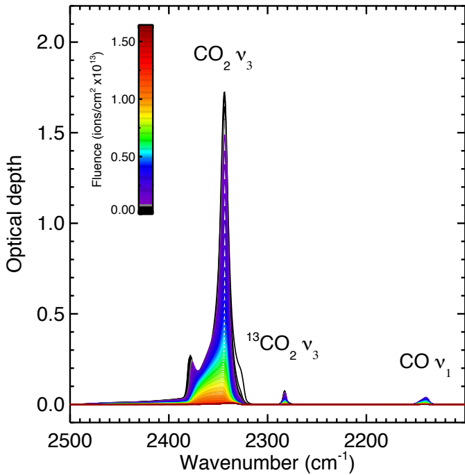
Fig. A.6. Infrared spectra for third CO 2 ice experiment with 58 Ni 9+ at 33 MeV ions.
