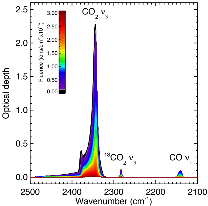
Fig. A.2. Infrared spectra for second CO 2 ice experiment with 40 Ca 9+ at 38.4 MeV ions.
