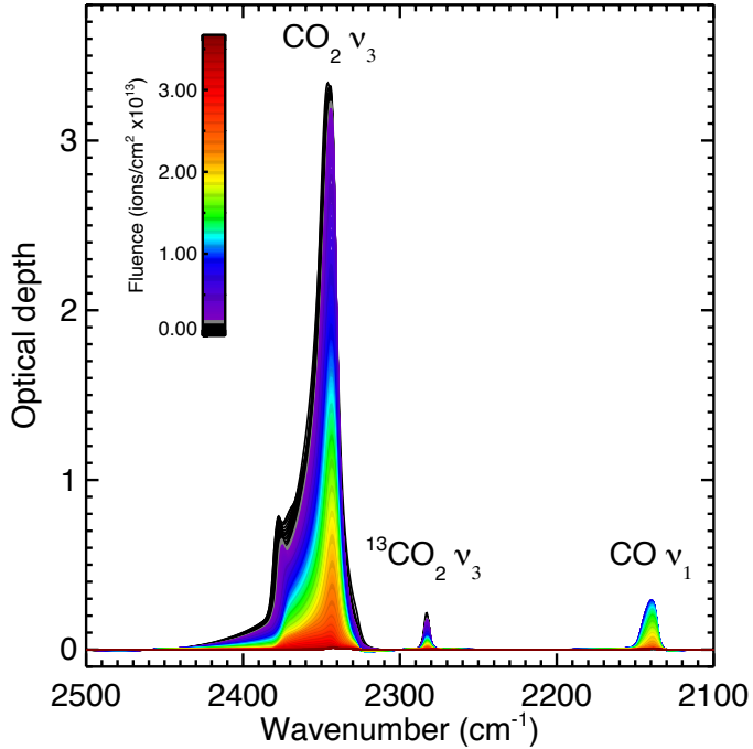
Fig. A.1. Infrared spectra for first CO 2 ice experiment with 40 Ca 9+ at 38.4 MeV ions. The inserted colour code gives the corresponding irradiation fluence.
