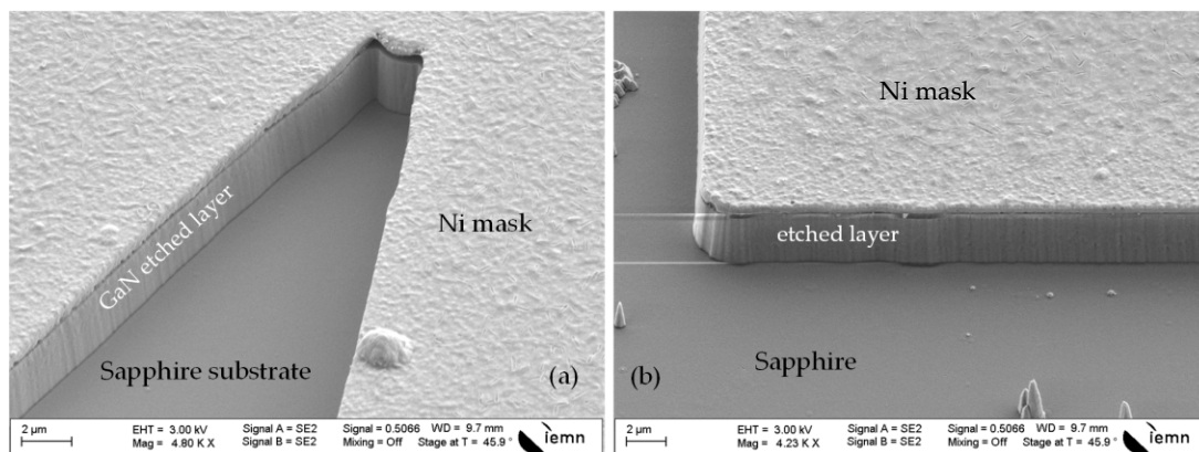
Figure 2. (a) Scanning electron microscope (SEM) analysis of mesa sidewalls after inductively coupled plasma (ICP) etching with sputtered nickel mask (depth of 3\ \mu\text{m} for ICP power of 500 Watts. (b) Typical etching results showing Ni mask.
