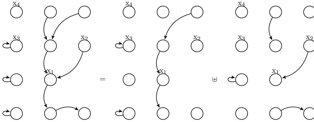
Figure 1. Disjoint memory states with one record field
