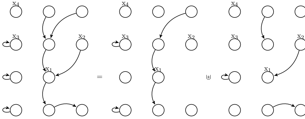
Figure 1. Disjoint memory states with one record field
