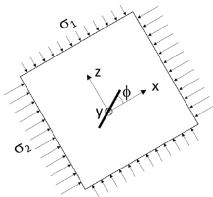
Figure 3 : Thin crack, placed in an infinite medium and subjected to a stress field ( \sigma_1 , \sigma_2 ) \Phi the angle of the crack with the x-axis.
