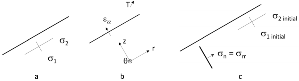
Figure 4 : Mechanical and thermo mechanical stresses: a - Mechanical stresses; b - Stresses / strain linked to thermal variations; c – Fracture perpendicular to the free surface submitted to tension and initial stresses
