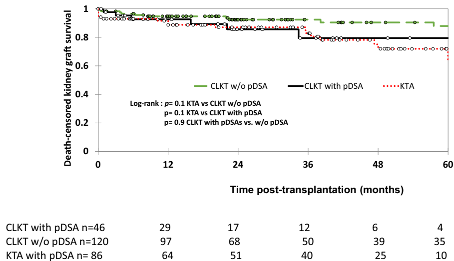
Figure 2. Death-censored kidney graft survival. CLKT, combined liver-kidney transplantation; KTA, kidney transplant alone; pDSA, preformed donor-specific anti-human leukocyte antigen antibody.
