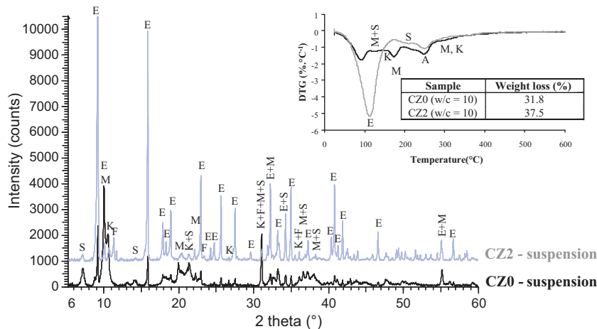
Fig. 10. X-ray diffraction and thermogravimetry analysis of cement suspensions prepared from CZ0 and CZ2 ( w/c ratio increased to 10, constant \text{Zn}/c ratio) after one week of stirring at 20 °C under nitrogen atmosphere. E, ettringite; F, Friedel's salt; K, Kuzel's salt; M, calcium monosulfoaluminate hydrate; S, strätlingite; A, \text{AH}_3 .
