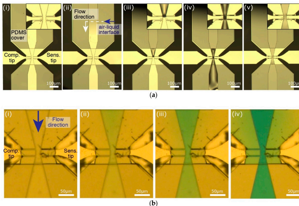
Figure 7. (a) After assembling the PDMS cover on the MEMS device (i); the formed channel is filled with liquid. Adjusting the pressure with the pump, the liquid enters the channel (ii); reaches the opposing tips (iii); goes through the handling area (iv); and finally, completely fills the channels; (b) The liquid exchange capability of the device is tested with water and a blue dye solution. (i) While the channel is filled with water; (ii,iii) a blue dye solution is injected at the inlet and within seconds (iv) the liquid in the channel is completely replaced.
