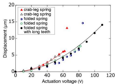
Figure 3. Actuation characteristics of various spring designs.
