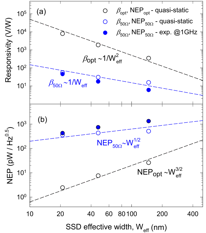
Figure 4. Log-log plot of the (a) responsivity and (b) NEP versus the effective channel width extracted with the quasi-static model from DC measurements (void symbols) and experimental measurements @1 GHz (solid symbols) of SSDs with N = 1 and L = 1 \mu\text{m} . The optimum and 50 \Omega values are plotted in both cases, obtained using the equations (1), (2) and (4). Dashed lines indicate the trends of the different magnitudes expected in the model of [11].
