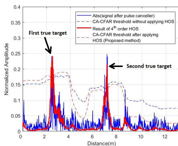
Fig. 11 Comparison of the CA-CFAR performance run directly on the signal without time-delay estimation and with time-delay estimation (HOS), P_{fa} = 10^{-5} , M = 150 and N = 2 . Two real targets present at 2.5 and 7 m away from the radar
