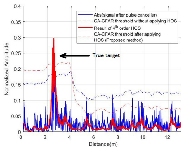
Fig. 10 Comparison of the CA-CFAR performance run directly on the signal without time-delay estimation and with time-delay estimation (HOS), P_{fa} = 10^{-5} , M = 150 , and N = 2 . A real target presents 2.5 m away from the radar
