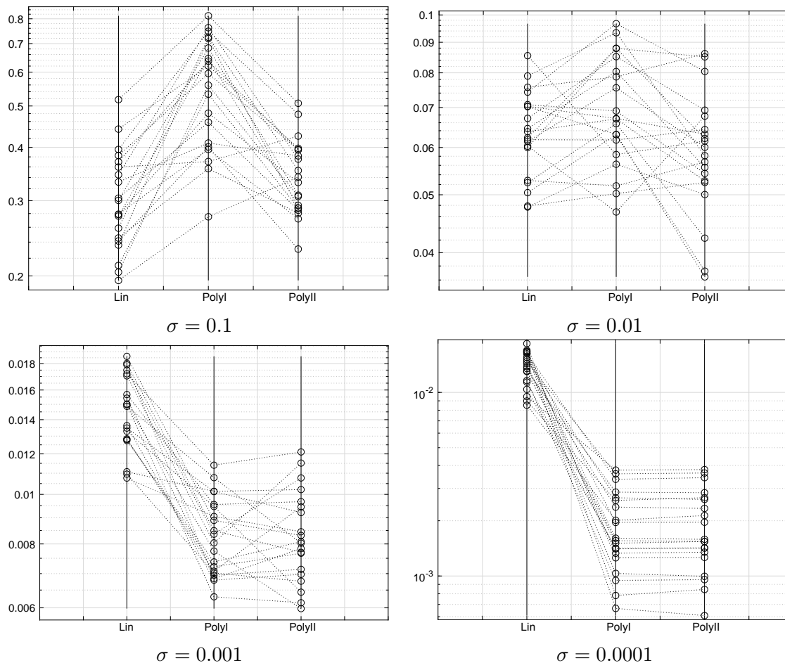
Figure 1: Recovery errors for near-optimal linear estimate (left) and for polyhedral estimates yielded by Proposition 4.2 ( PolyI , middle) and by the construction from Section 3 ( PolyII , right), 20 simulations per each value of \sigma .
