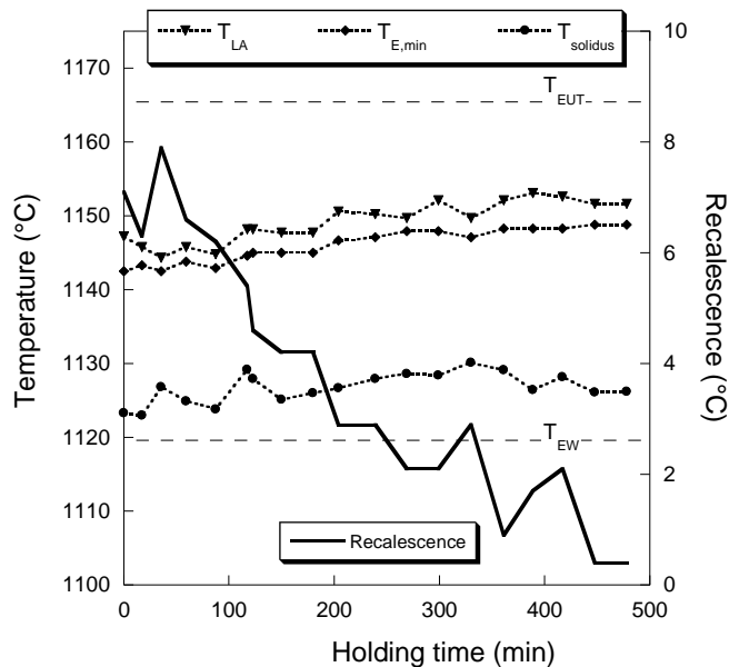
Figure 5. Evolution of the characteristic temperatures and of recalescence during holding for inoculated alloys.
