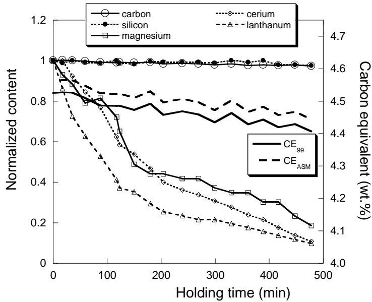
Fig. 1 – Effect of holding time on the content of the melt in C, Si, Mg, Ce and La relative to the composition of the first sample, and of the calculated carbon equivalent CE according to the two equations (1) and (1').
