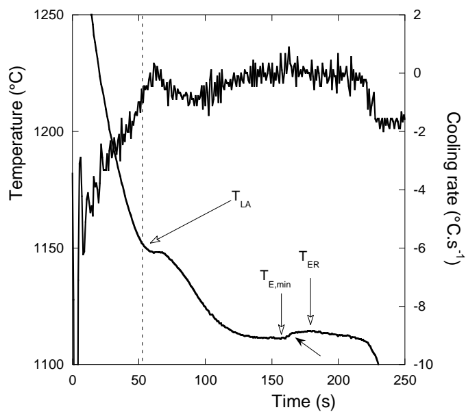
Figure 2. Typical example of cooling curve and its time derivative (non-inoculated Q alloy) with definition of the characteristic temperatures (open arrows), see text. The solid arrow indicates an abrupt recalescence which is referenced to later in the main text.
