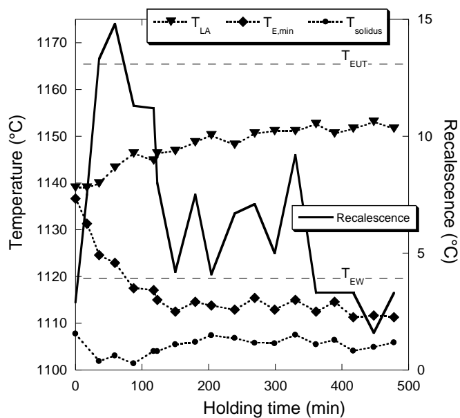
Figure 8. Evolution with holding time of the characteristic temperatures and of recalescence for the non-inoculated samples.
