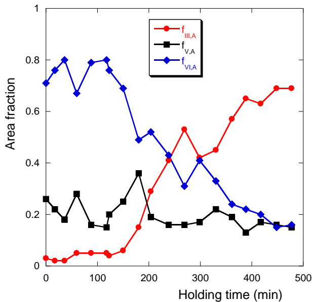
Figure 4. Change with holding time of the relative fractions of graphite, f_{III-A} , f_{V-A} and f_{VI-A} , for all inoculated samples. After Regordosa et al. [19].
