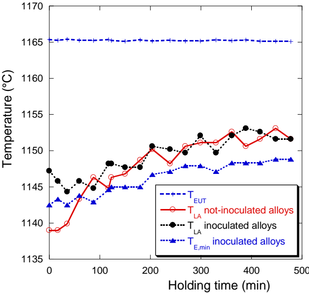
Figure 9. Evolution with holding time of T_{EUT} (calculated from the non-inoculated alloys' composition), of T_{E,min} and T_{LA} for inoculated samples, and of T_{LA} for non-inoculated samples.
