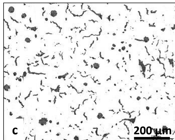
Figure 3. Inoculated samples: cooling curves of trials A and S (a), and micrograph of samples A_{inoc} (b) and S_{inoc} (c). The open arrow shows the minimum temperature in the plateau of curve S (see text for details).
