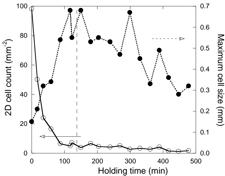
Figure 10. Evolution with holding time of the number and size of compact graphite cells in non-inoculated alloys.
