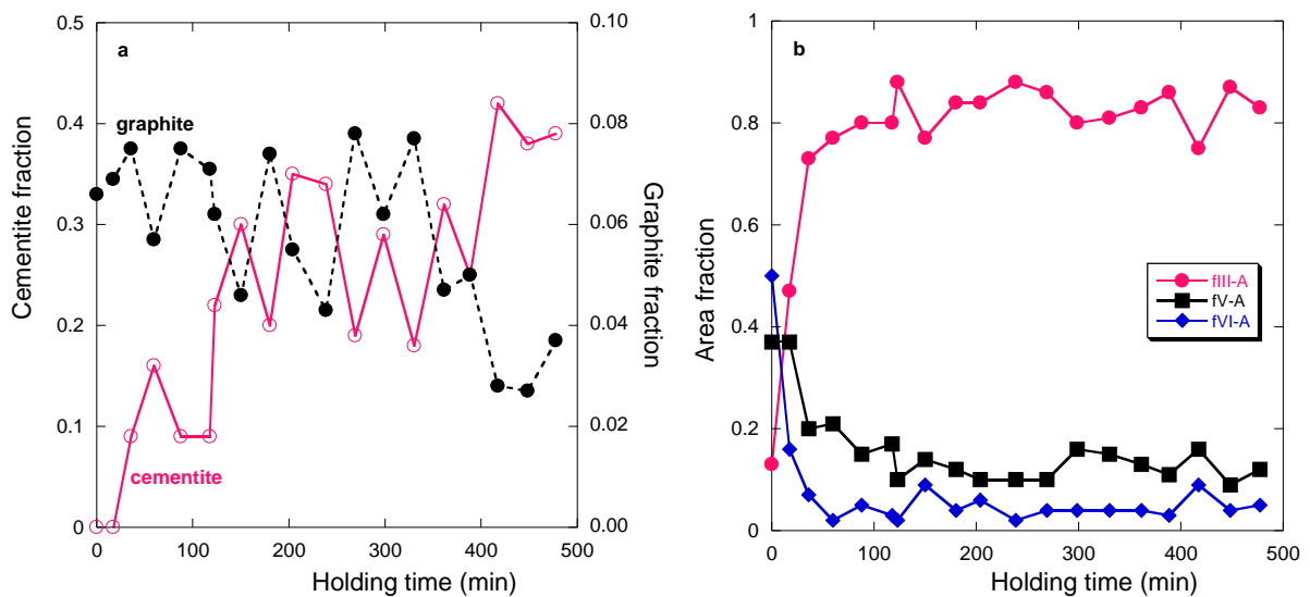
Figure 7. Evolution with holding time of the amount of graphite and cementite (a) and of the relative fractions f_{III-A} , f_{V-A} and f_{VI-A} (b) in the non-inoculated samples. After Regordosa et al. [19].
