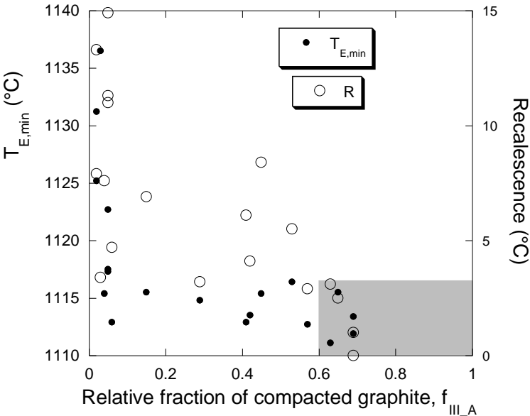
Figure 11. Correlation between the relative amount of compact graphite, f_{III\_A} , in inoculated samples with the values of T_{E,min} and R in the corresponding non-inoculated sample. The greyed area corresponds to inoculated alloys with compact graphite.
