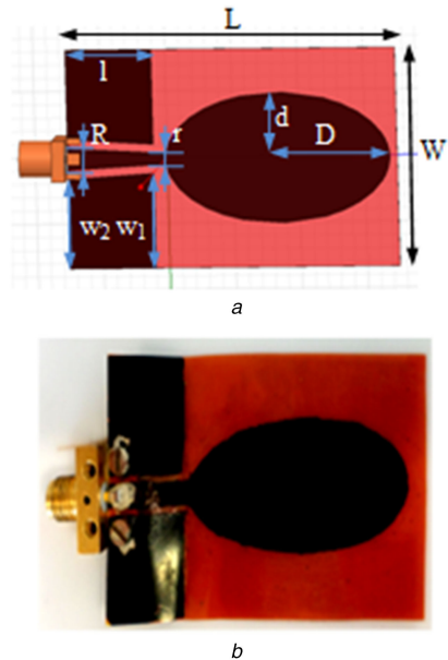
Fig. 3 Uncrumpled antenna designed on the kapton substrate (a) HSSFF® layout view, (b) Photograph of the realised antenna
