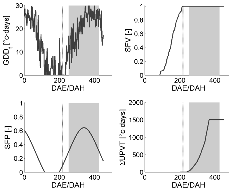
Figure 4: Simulated GDD_t (Growing-Degree-Day), SFV (Slowdown Factor accounting for Vernalization), SFP (Slowdown Factor accounting for Photoperiod ) and UPVT (Photo-Vernalo-Thermic Units) for the Salina US site (calibration site) over the season 2017 (second growing year). Light grey dashed line represents the day where cold requirements is fully met. Light grey shaded area represents the period for which SFP is greater than 0.3 (>11h daylength). UPVT accumulation was stopped when maturity was reached.
