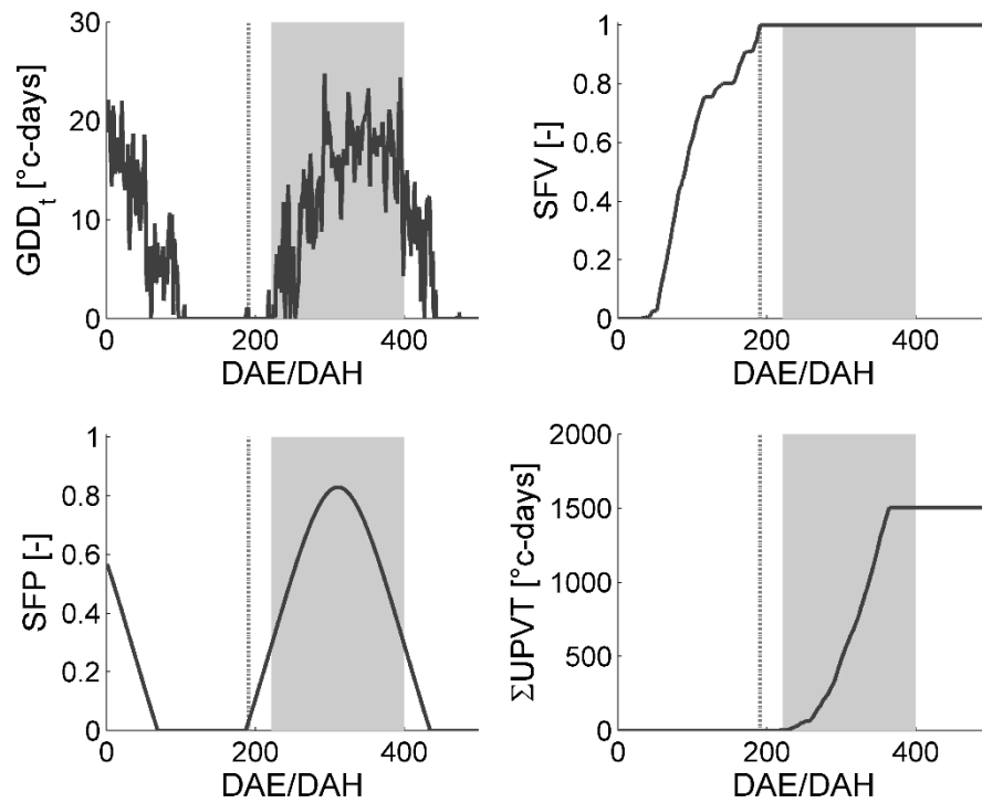
Figure 3: Simulated GDD_t (Growing-Degree-Day), SFV (Slowdown Factor accounting for Vernalization), SFP (Slowdown Factor accounting for Photoperiod ) and UPVT (Photo-Vernalo-Thermic Units) for the Carman-LN Canadian site (validation site) over the season 2017 (second growing year). Light grey dashed line represent the day where cold requirement is fully met. Light grey shaded area represent period for which SFP is greater than 0.3 (>11h daylength). UPVT accumulation was stopped when maturity was reached.
