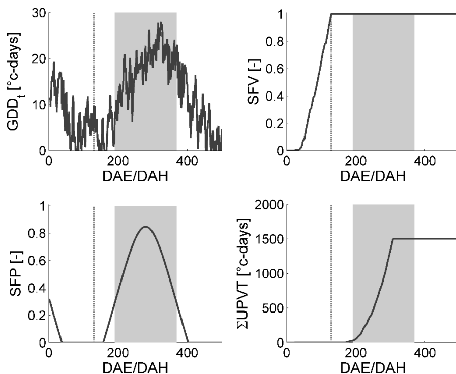
485 486 Figure 2: Simulated GDD_t (Growing-Degree-Day), SFV (Slowdown Factor accounting for Vernalization), SFP (Slowdown 487 Factor accounting for Photoperiod) and UPVT (Photo-Vernal-Thermic Units) for the Maubec French site (validation site) 488 over the season 2018 (establishment year). Light grey dashed line represents the day where cold requirement is fully met. 489 Light grey shaded area represents the period for which SFP is greater than 0.3 (>11h daylength). UPVT accumulation was 490 stopped when maturity was reached.
