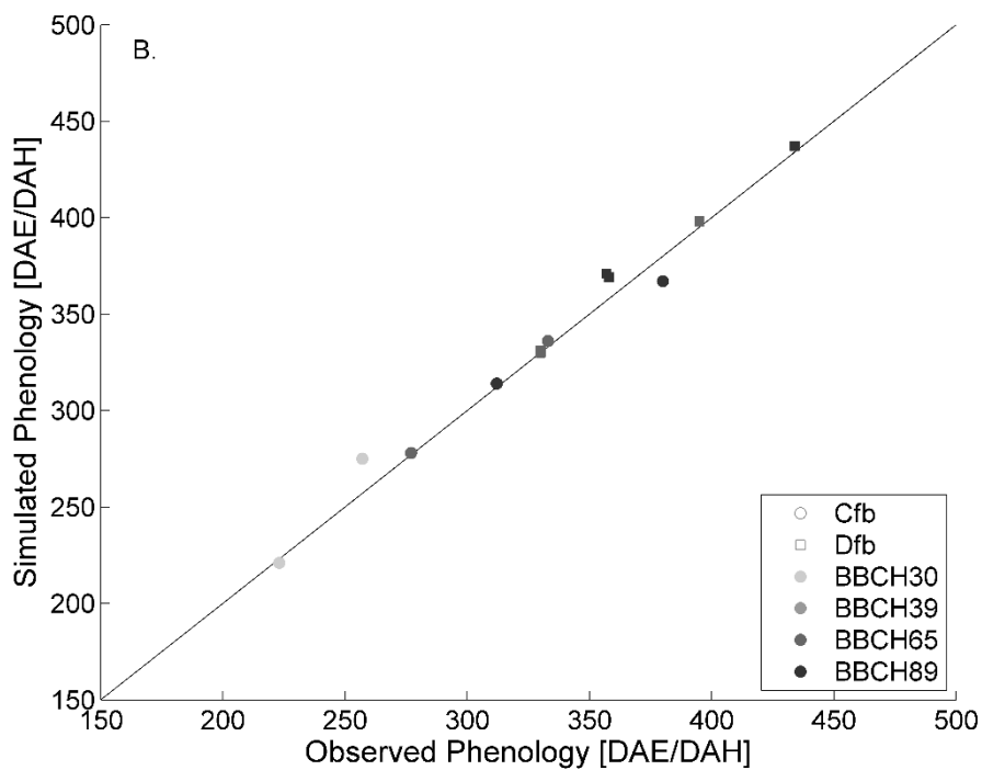
Figure 1: Observed and simulated phenology for the calibration (A) and validation (B) datasets. Climate type Cfb is represented by circles (o), climate type Dfb is represented by squares (□) and climate type Dfa is represented by triangle (Δ). Intensity of grey varies with simulated crop stage in BBCH scale, with lighter grey being stem extension (BBCH 30) and darker grey being maturity (BBCH 89).
