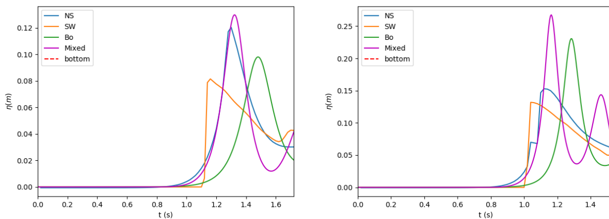
FIGURE 10. Comparison between the three fluid mechanics models and the proposed mixed shallow water/Boussinesq model, for two test cases at the probe x = 2.25 m.
