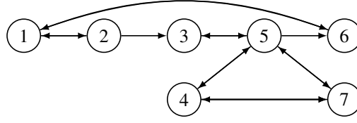
Fig. 6: Attack graph of AF .
