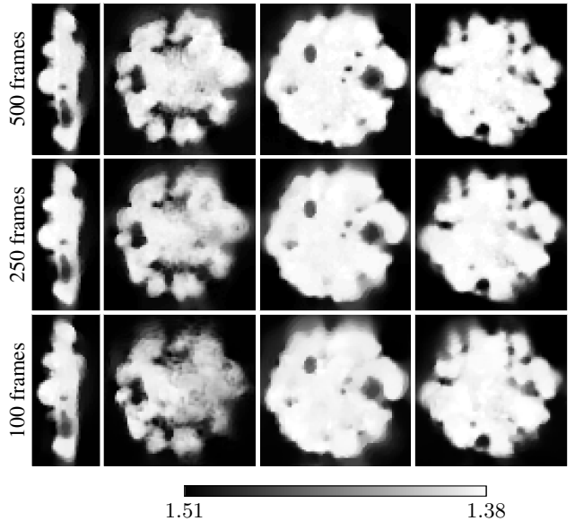
Fig. 4: Top: relative error for different settings. From left to right: initial guess, Lippmann-Schwinger model from complex measurements and 1000 frames, Lippmann-Schwinger model from intensity measurements and 1000, 500, 250, and 100 frames, respectively. Bottom: reconstructions of the RI volume with Lippmann-Schwinger model from intensity measurements and 500, 250, and 100 frames. The axial positions are provided in Figure 3.
