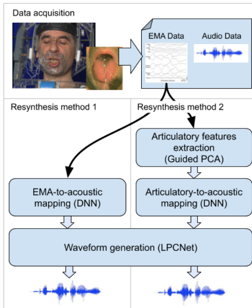
Figure 1: System overview. Two methods for synthesis from articulatory data we investigated: Method 1 predicts a target cepstrum from raw EMA data, i.e., a 12-dimensional feature vector, while Method 2 first reduces it to a vector of 6 articulatory components (JH, TB, TD, TT, LH, LP).
