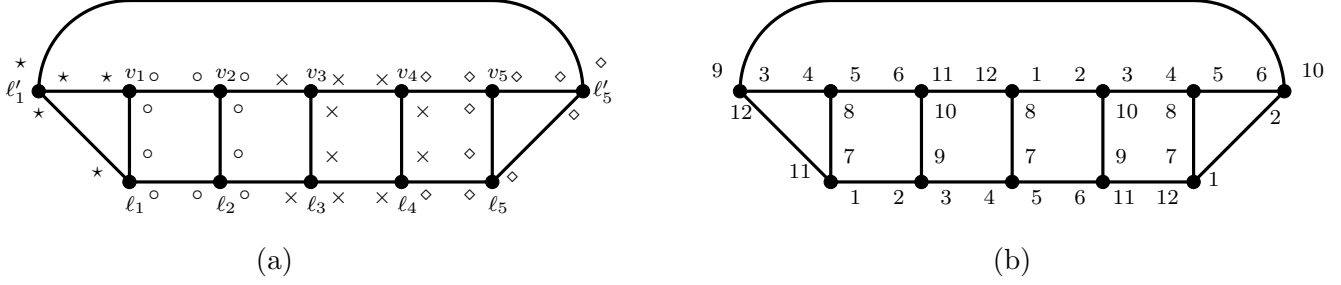
Figure 10: The necklace N_5 (for the proof of Theorem 14).
