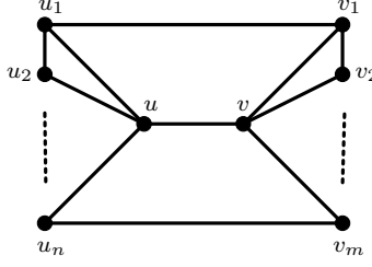
Figure 12: The Halin graph HD_{m,n} .
