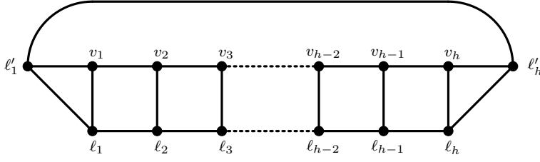
Figure 5: The graph N_h .
