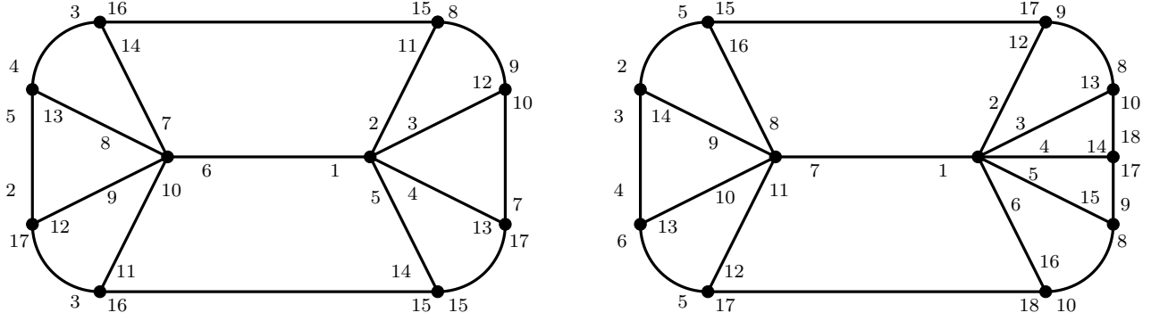
Figure 17: Strong incidence colourings of HD_{4,4} and HD_{5,4} .
