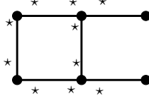
Figure 3: The graph L .
