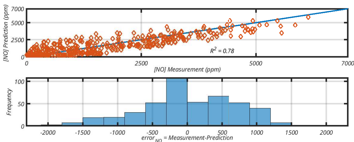
Figure 10. Comparison between [NO] measurement and [NO] prediction based on [NO] model.
