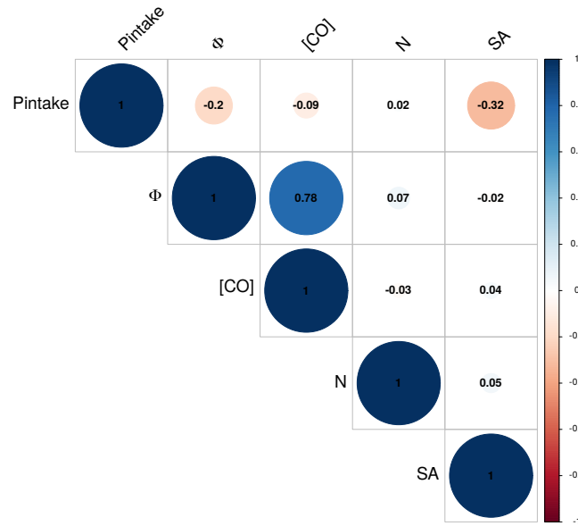
Figure 3. Correlogram of CO emission with governing parameters.
