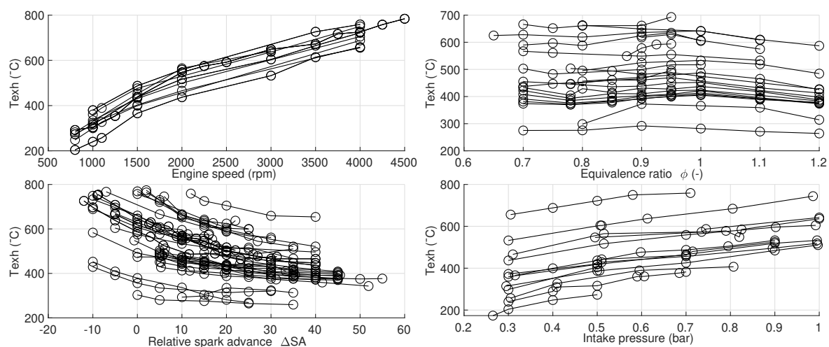
Figure 16. Exhaust temperature as a function of control parameters (each curve represents a series of measurements where only the parameter in abscissa changes).
