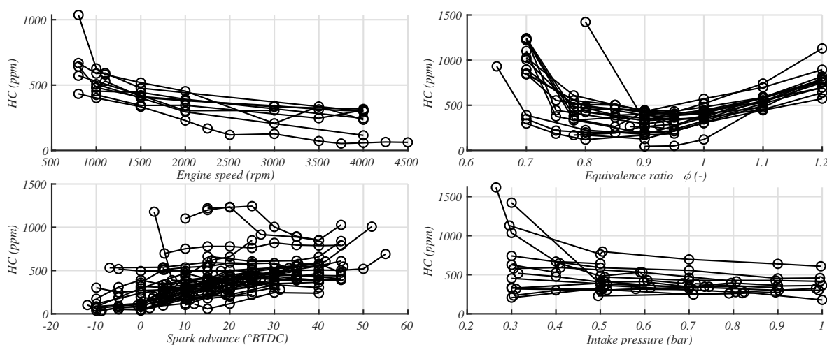
Figure 5. HC concentration as a function of control parameters (each curve represents a series of measurements where only the parameter in abscissa changes).
