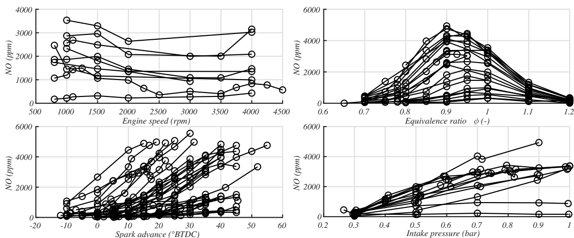
Figure 8. NO concentration as a function of control parameters (each curve represents a series of measurements where only the parameter in abscissa changes).
